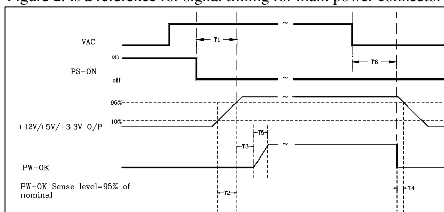
Figure 2. PS-OK Timing Sequence
