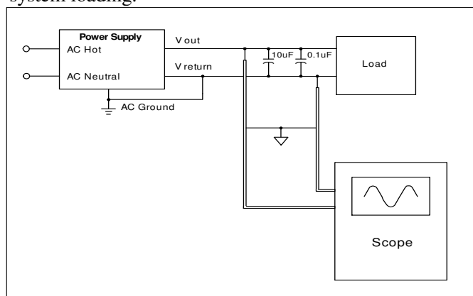
Figure 1. Ripple voltage test circuit
