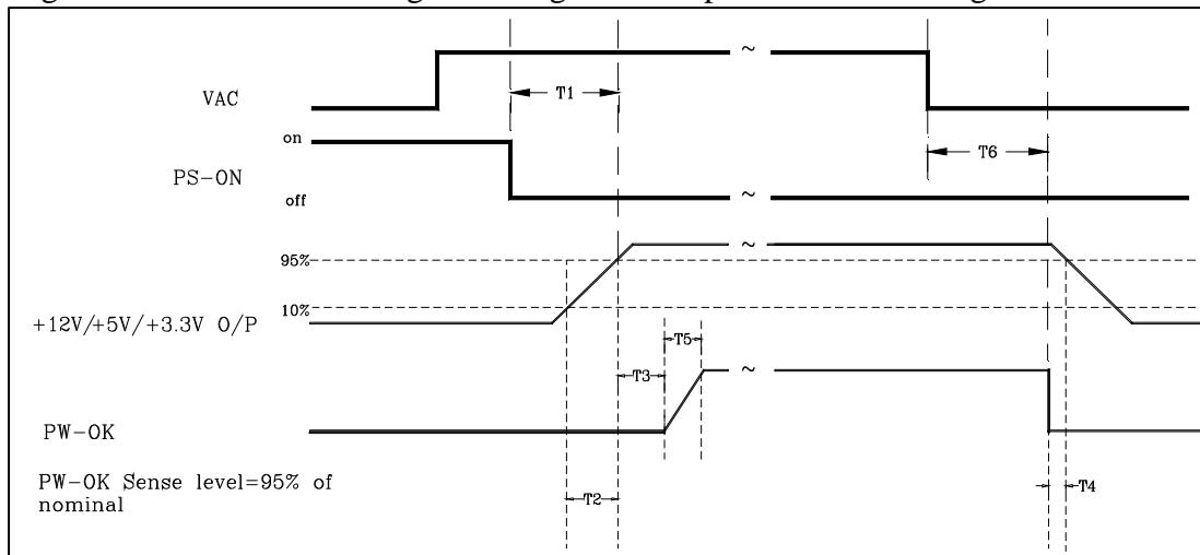
Figure 2. PS-OK Timing Sequence
