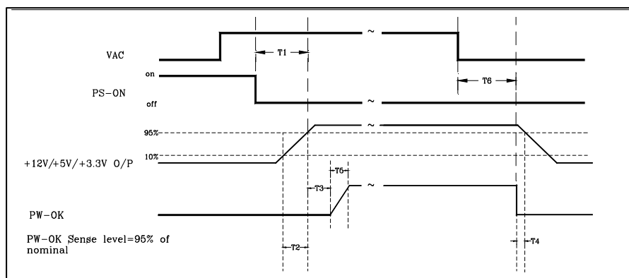
Figure 4. PS-OK Timing Sequence
