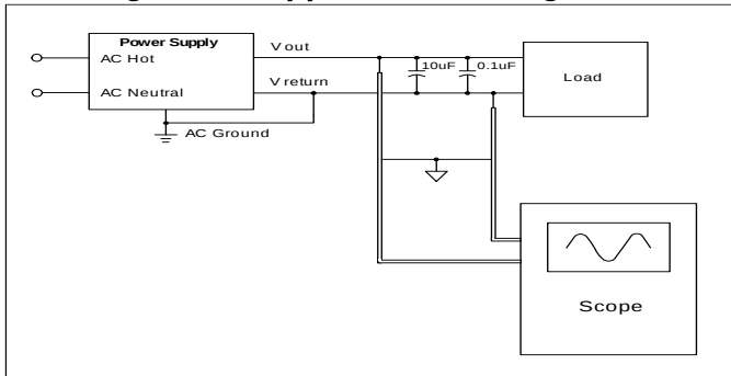
Figure 3. Ripple/Noise voltage test circuit
