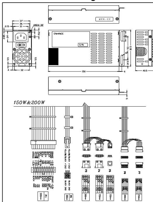
With 0/1 Switching
