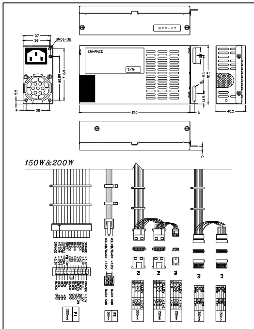
With 0/1 Switching
