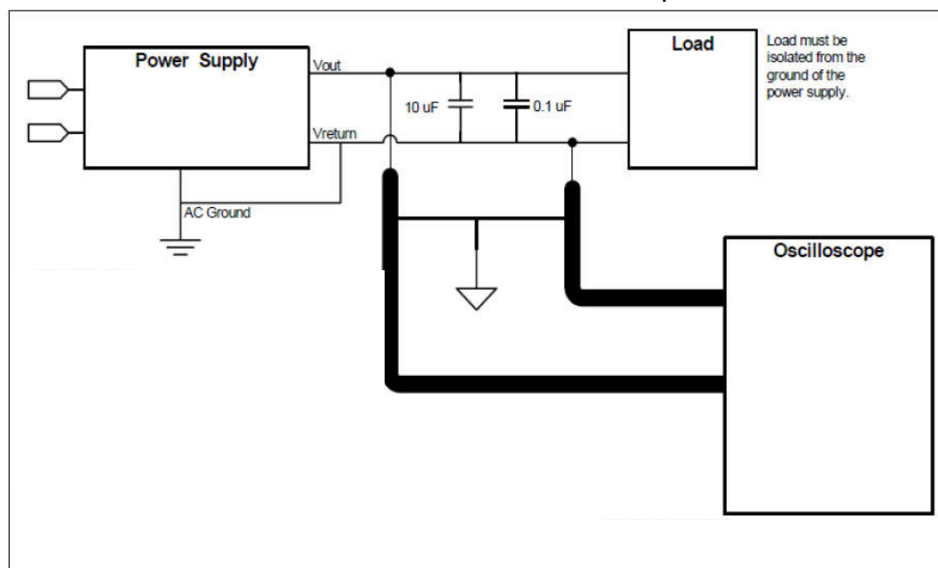
Differential noise test setup
