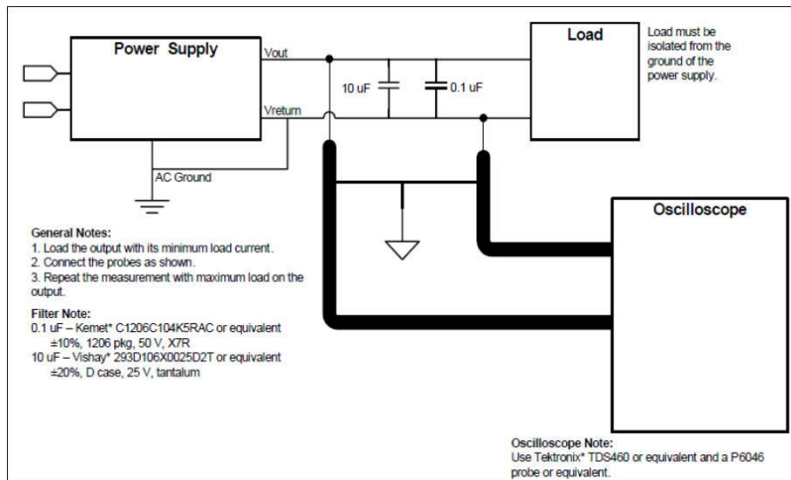
Differential noise test setup
